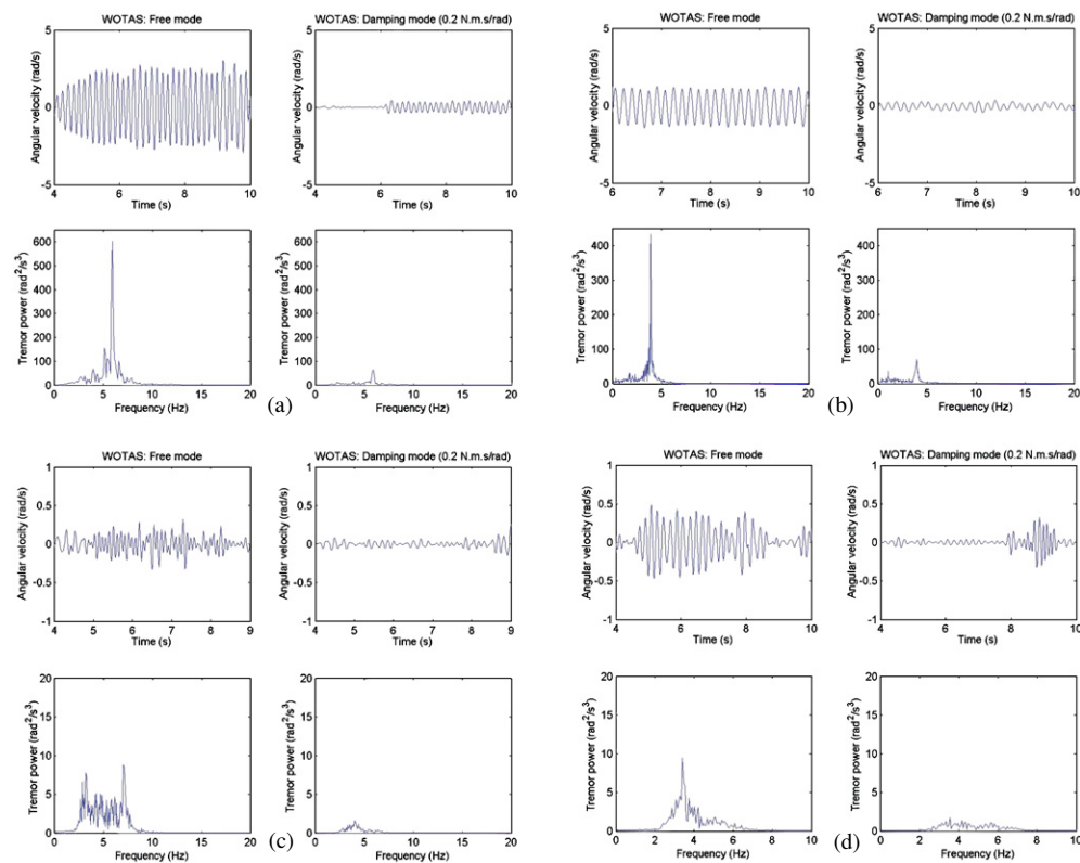
Figure 3. This figure illustrates the oscillations of the wrist with the associated power spectral density (PSD) of tremor with the motor in a free mode (left panels) and providing viscosity of 0.2 \text{ N ms rad}^{-1} (right panels) in one of the patients. Note the strong reduction in the PSD when viscosity is applied. Oscillations are expressed in \text{rad s}^{-1} and PSD is expressed in \text{rad}^2 \text{ s}^{-3} . (a) Reduction of postural tremor of the wrist with WOTAS, (b) reduction of postural tremor of the elbow with WOTAS, (c) reduction of kinetic (intention) tremor at the elbow with WOTAS, (d) reduction of tremor at the elbow level in a patient performing a finger-to-nose task.
